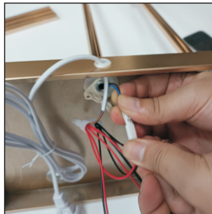
2. 66CM long lamp wire, through the 60CM long tube, install the lamp holder in one side, then install the tube on the position 2, and lock the power port on the back of the base
