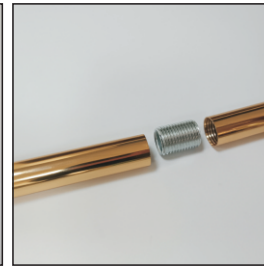
5. 126CM long lamp wire, through the 60CM long tube, install the lamp holder in one side, then install the tube on the position 5, and lock the power port on the back of the base
