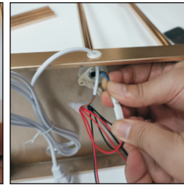
4. 106CM long lamp wire, through the 50CM long tube, install the lamp holder in one side, then install the tube on the position 4, and lock the power port on the back of the base
