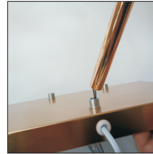
3. 86CM long lamp wire, through the 80CM long tube, install the lamp holder in one side, then install the tube on the position 3, and lock the power port on the back of the base
