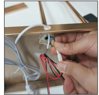
3. 86CM long lamp wire, through the 80CM long tube, install the lamp holder in one side, then install the tube on the position 3, and lock the power port on the back of the base
